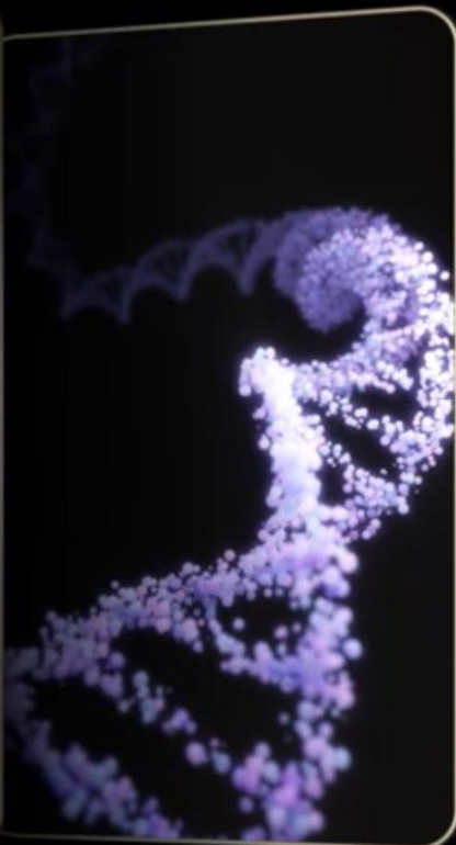
Parabricks Genomics
